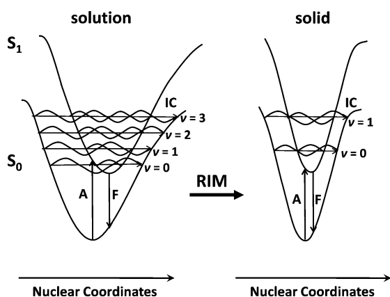
Figure 6. Sketch of the potential-energy surfaces of low-frequency twisting modes for CD-7 in solution and in the solid phase (RIM = restriction of intramolecular motion).
