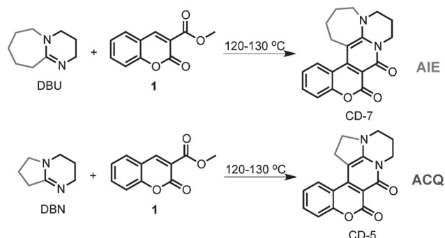
Scheme 1. Synthesis of CD-7 and CD-5.
